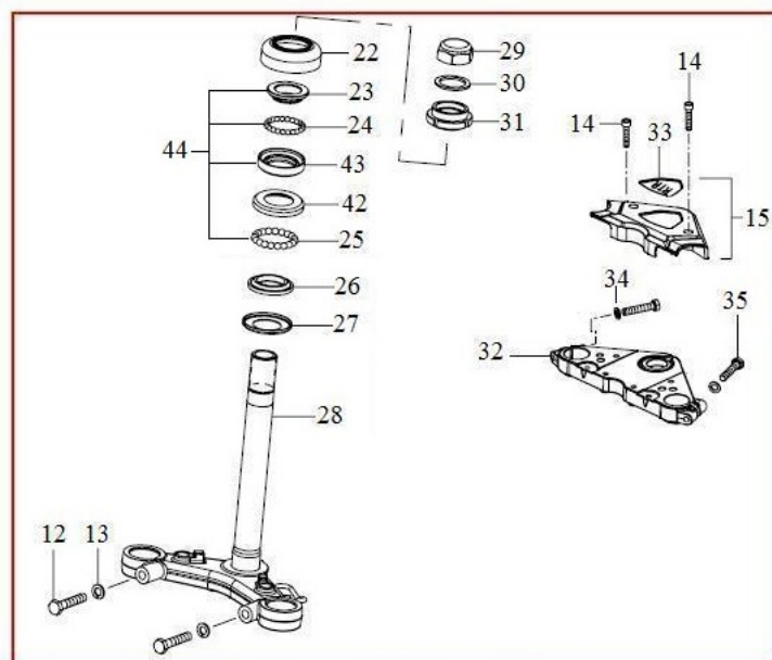
CANOTE E MESA SUPERIOR
